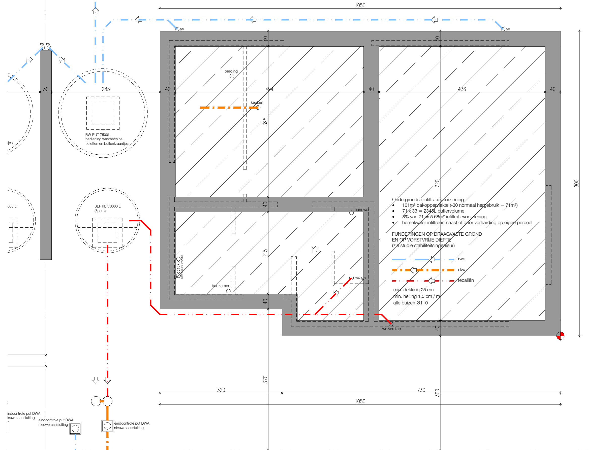
riolerings- en funderingsplan lot 39 81.76 m 2 bruto opp.
