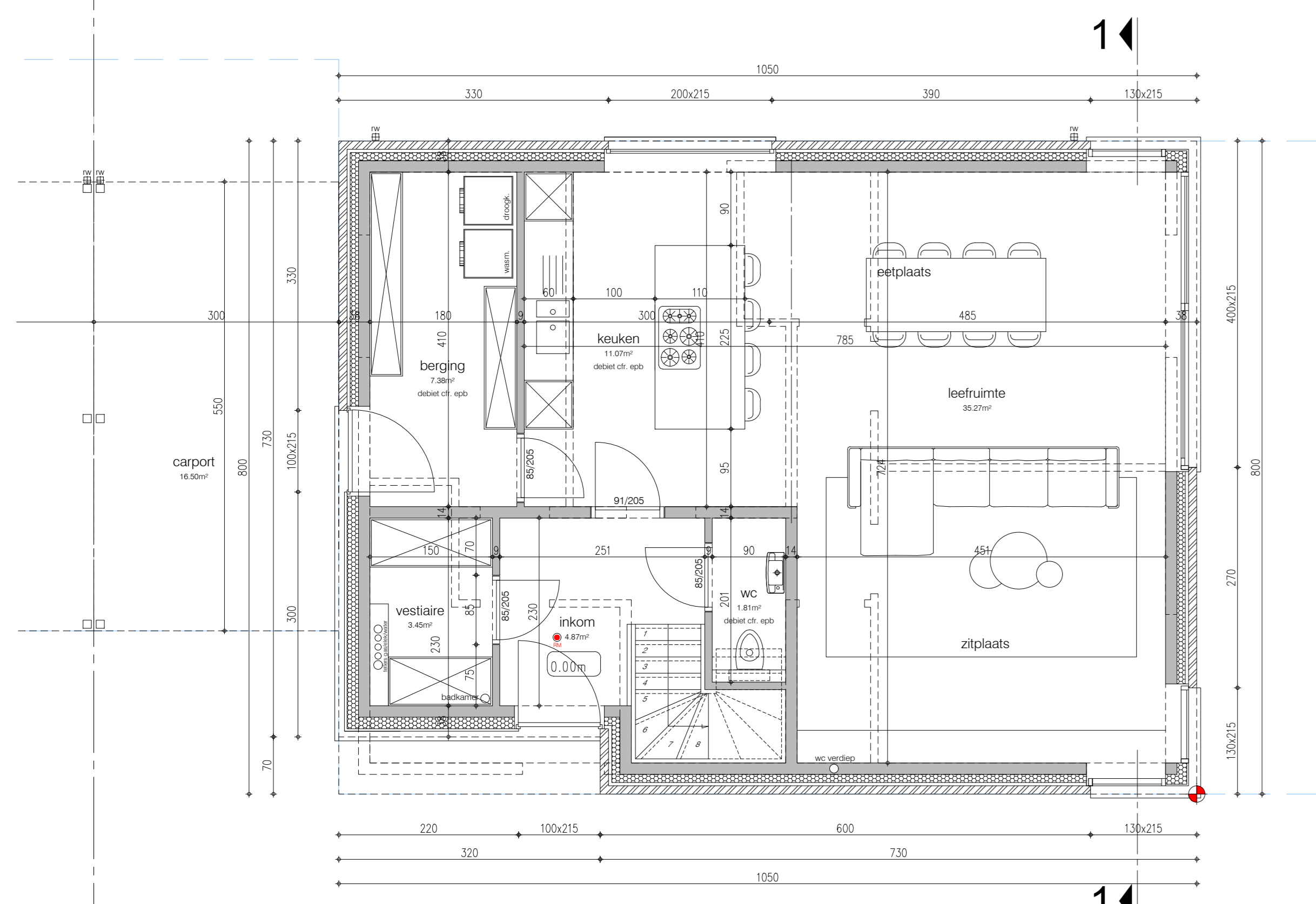
gelijkvloers lot 39 81.76 m 2 bruto opp. 68.27 m 2 netto opp.
