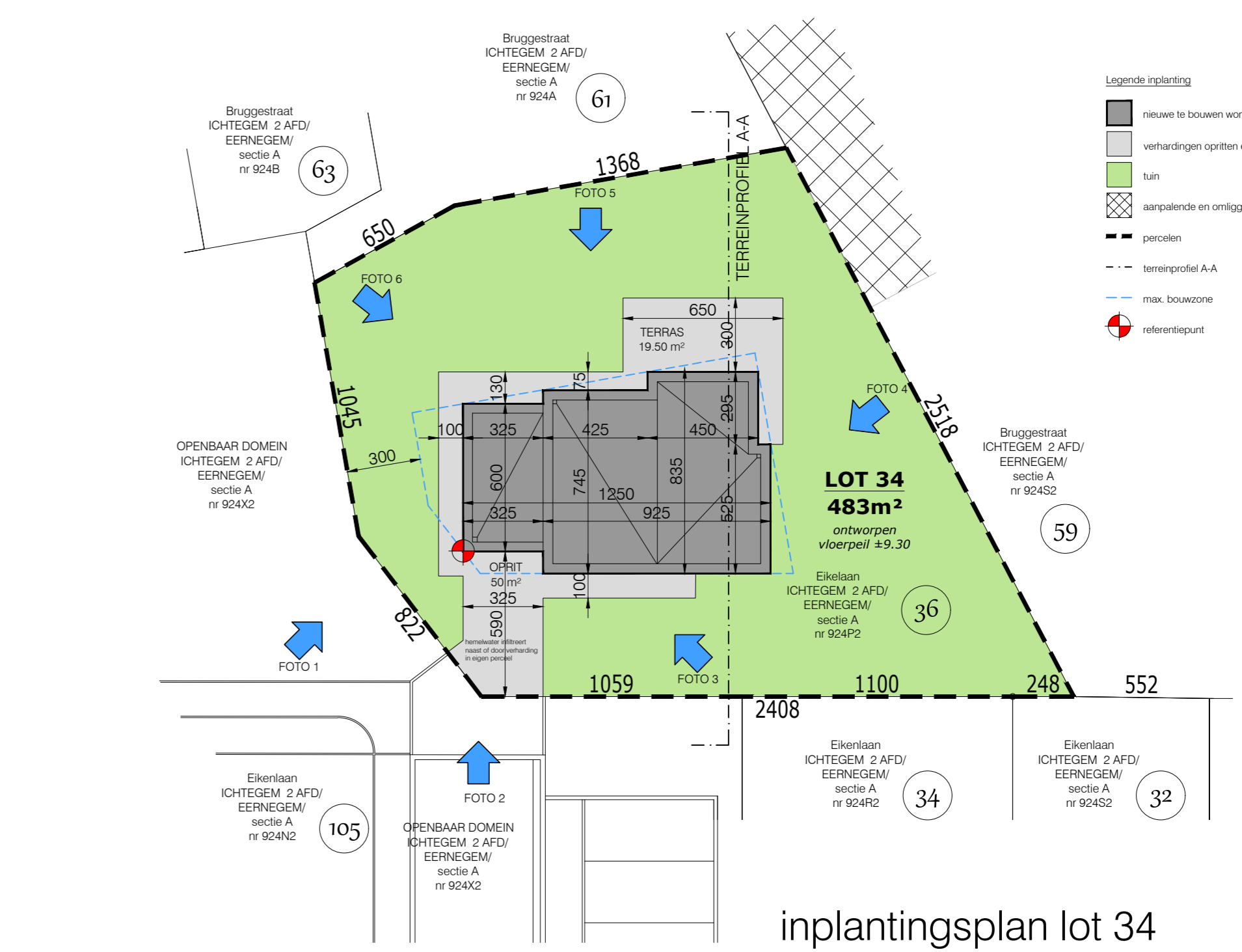
inplantingsplan lot 34
