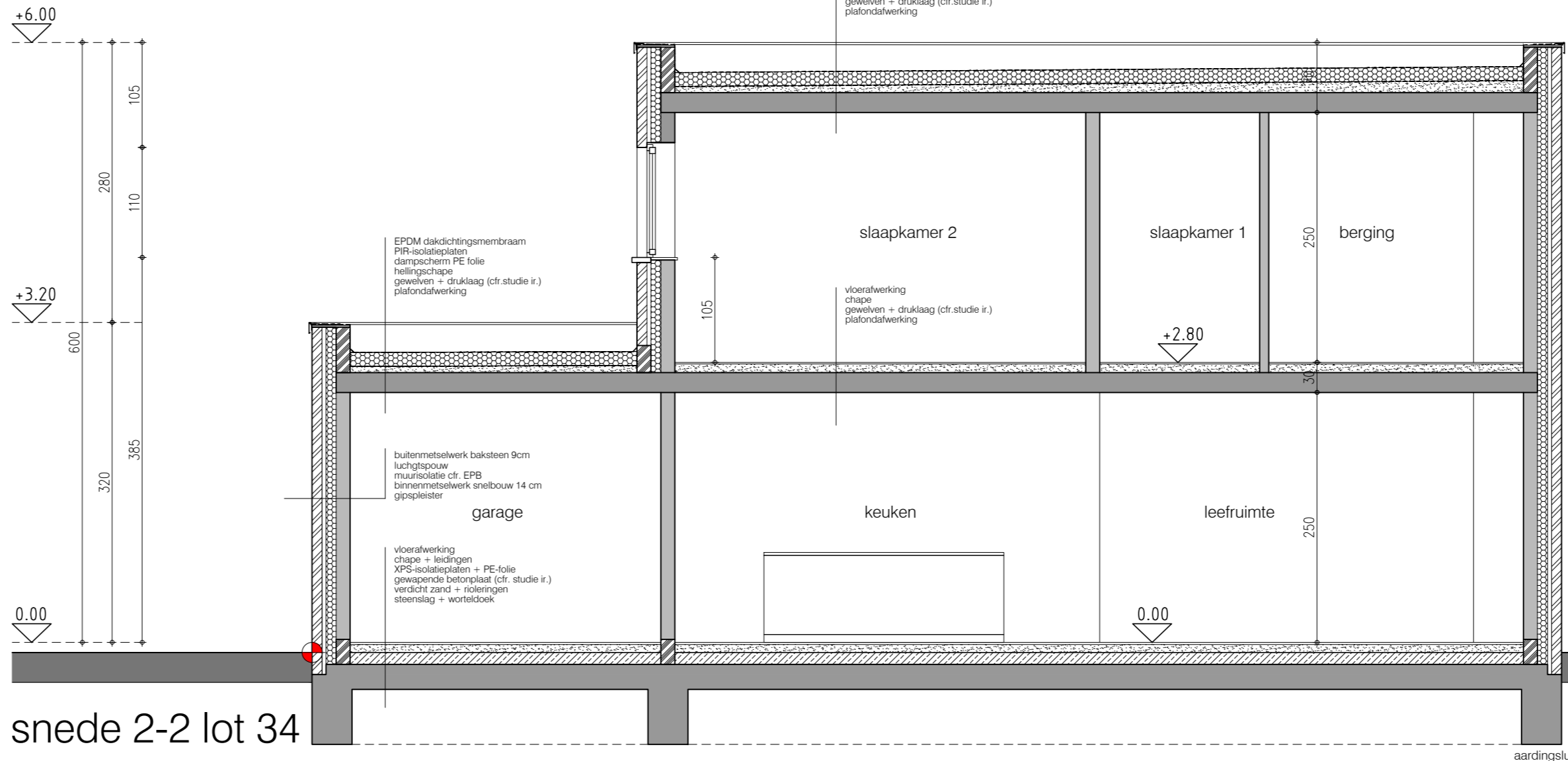
snede 2-2 lot 34
