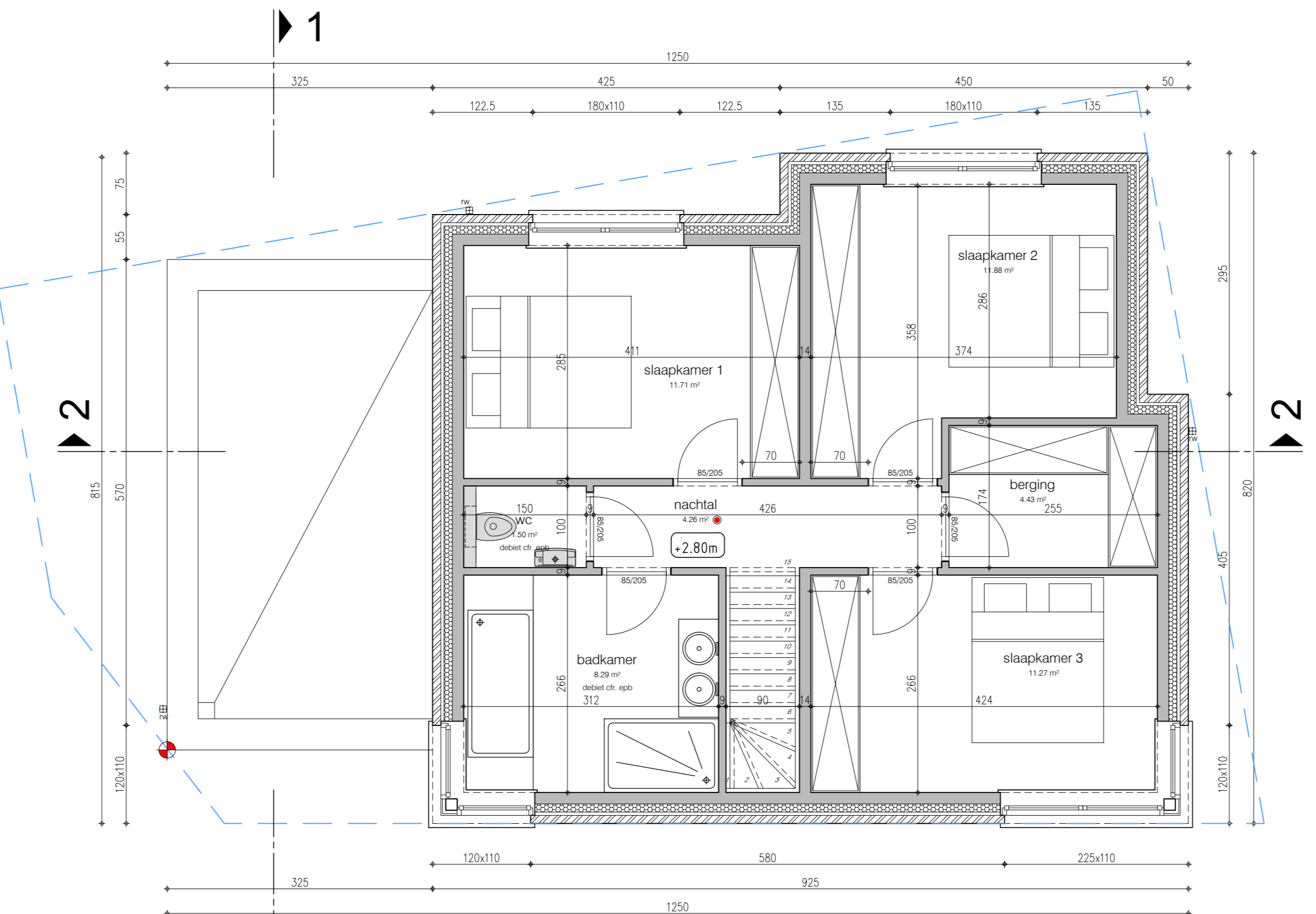
verdiepingsplan lot 34 bruto opp. 71.18 m 2
