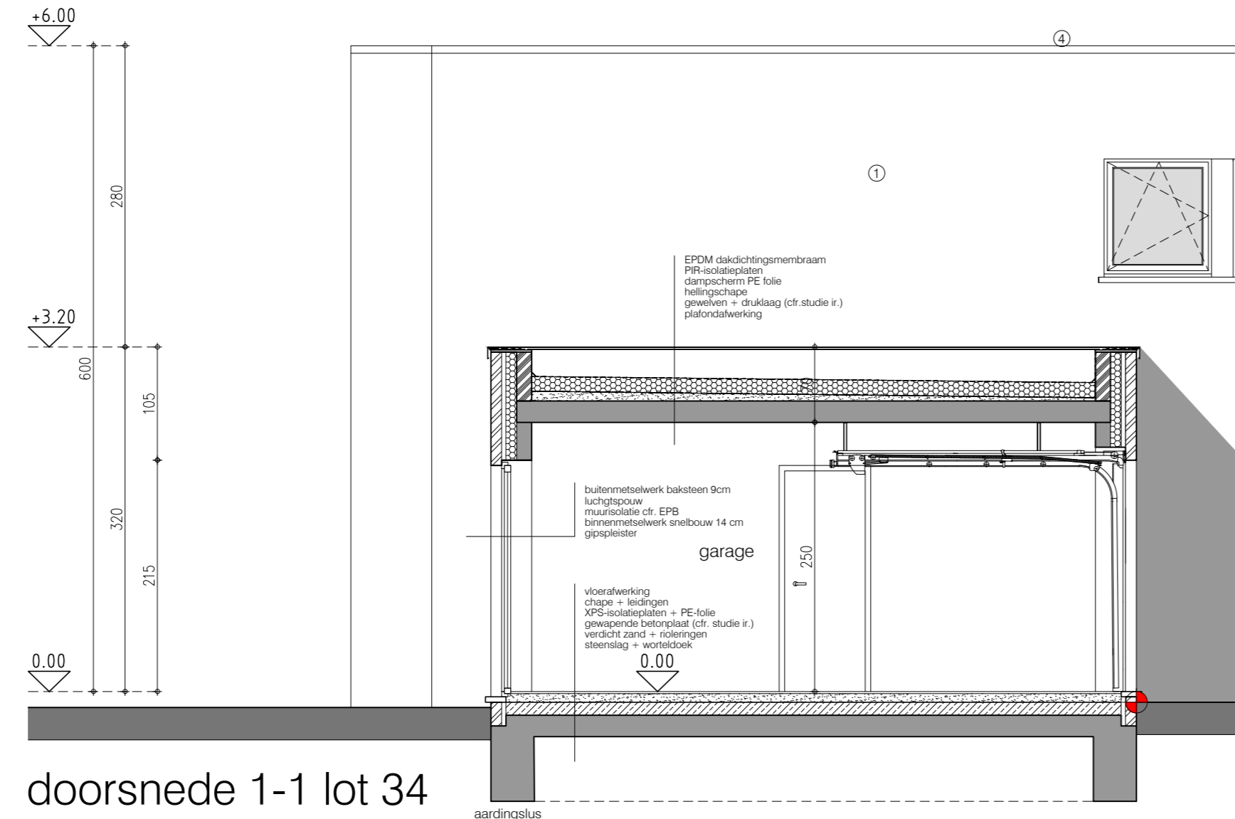
doorsnede 1-1 lot 34
