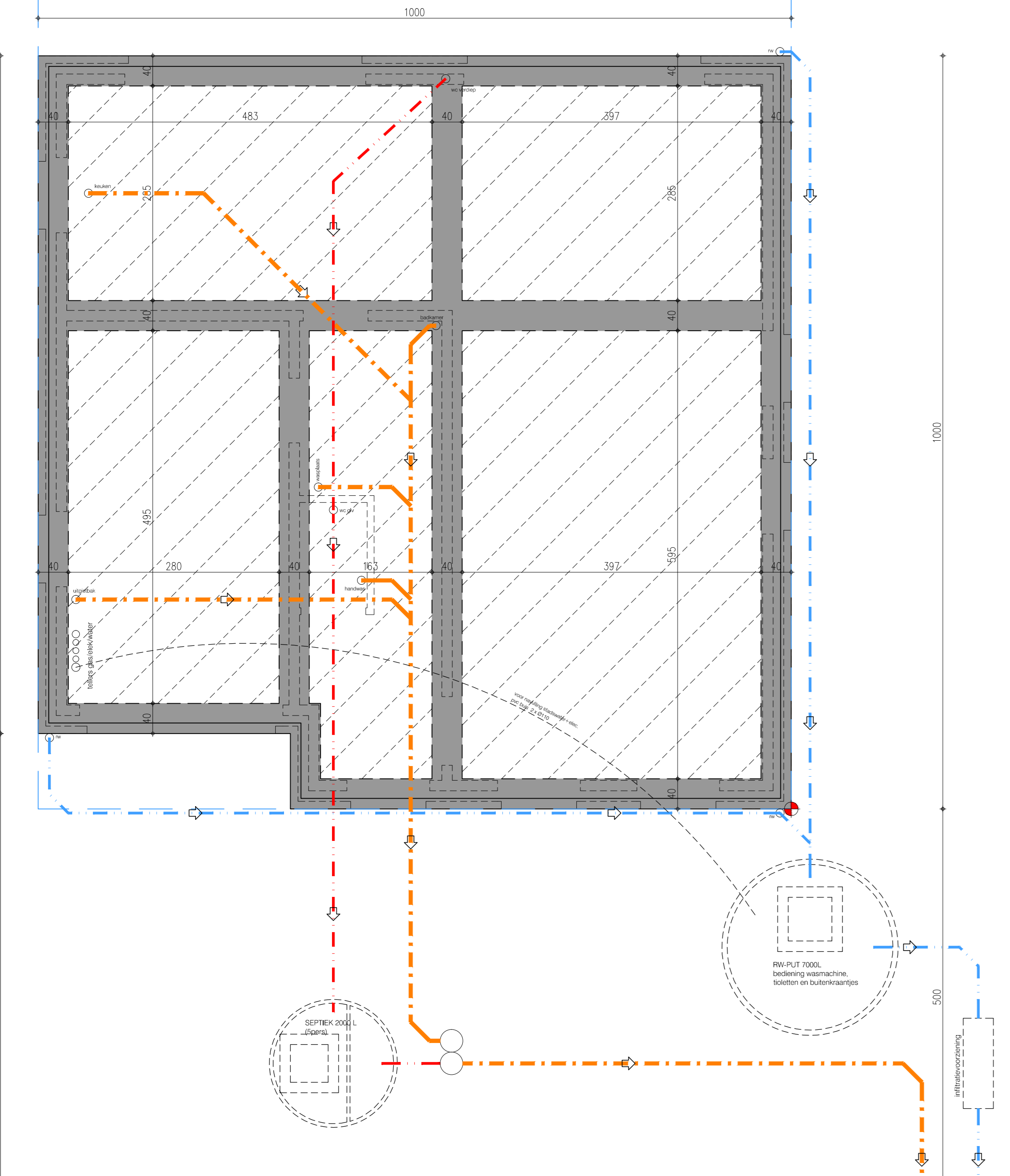
funderingsplan lot 4
