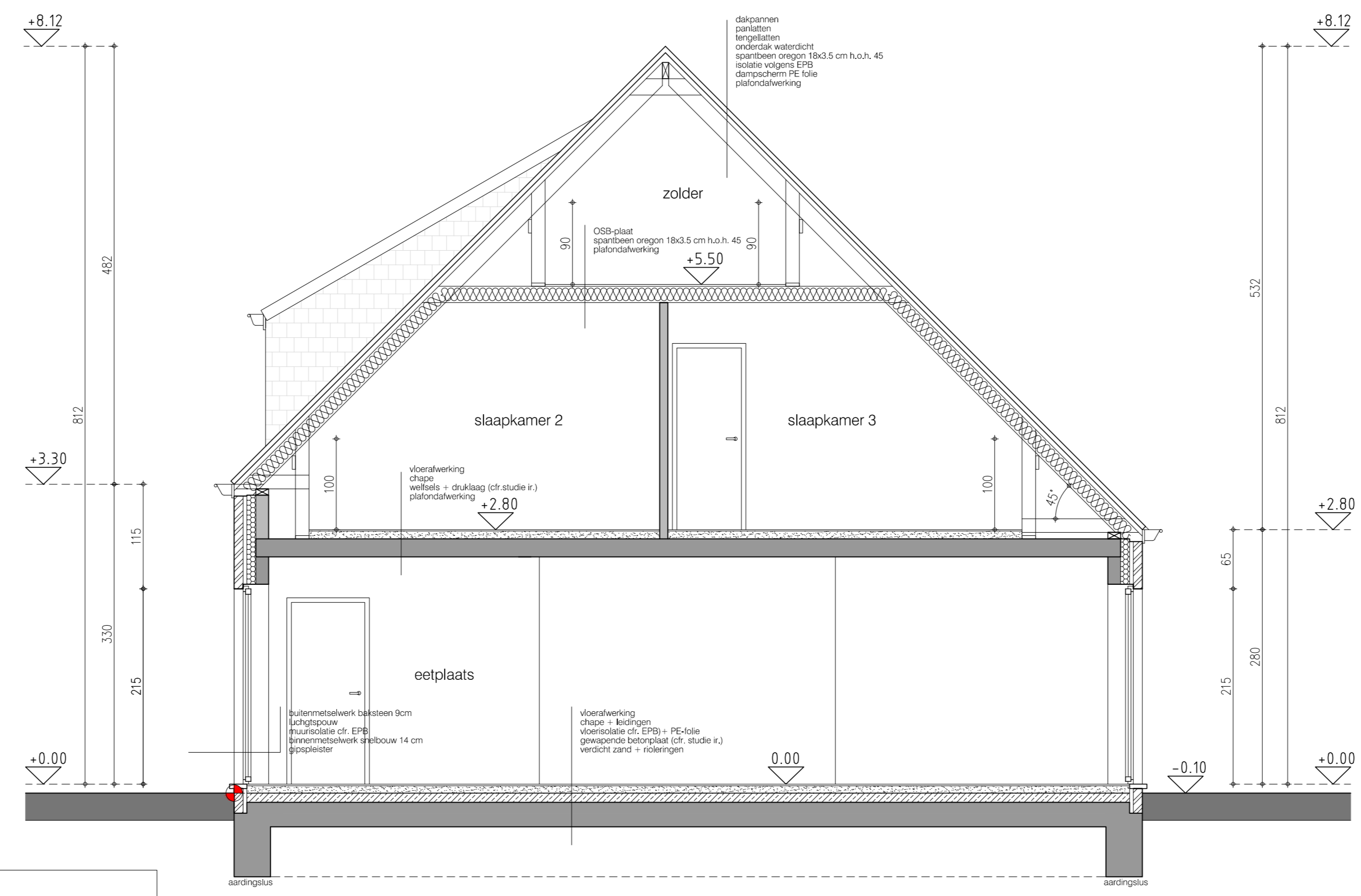
doorsnede 1-1 lot 4
