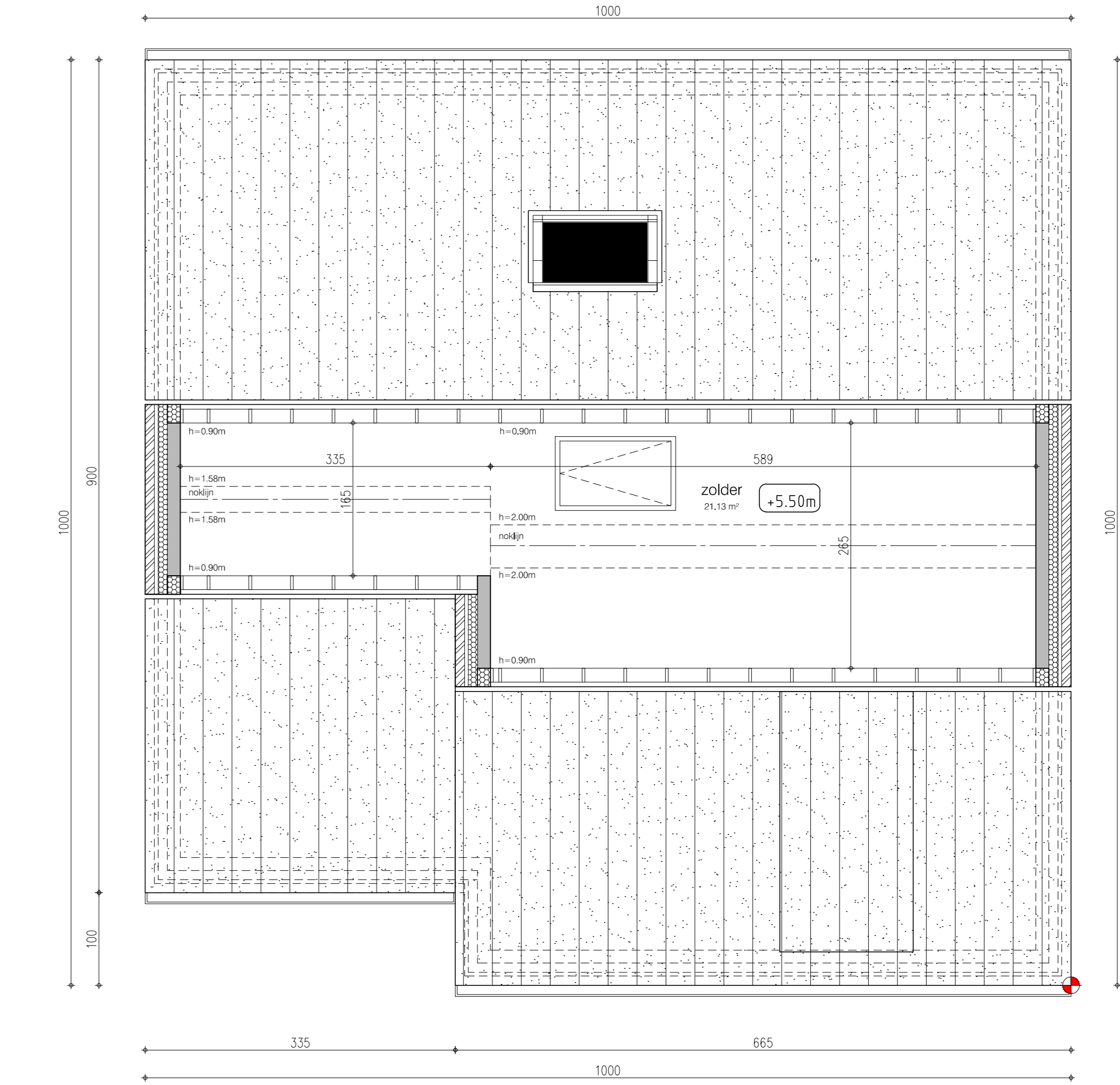
zolderplan lot 4
