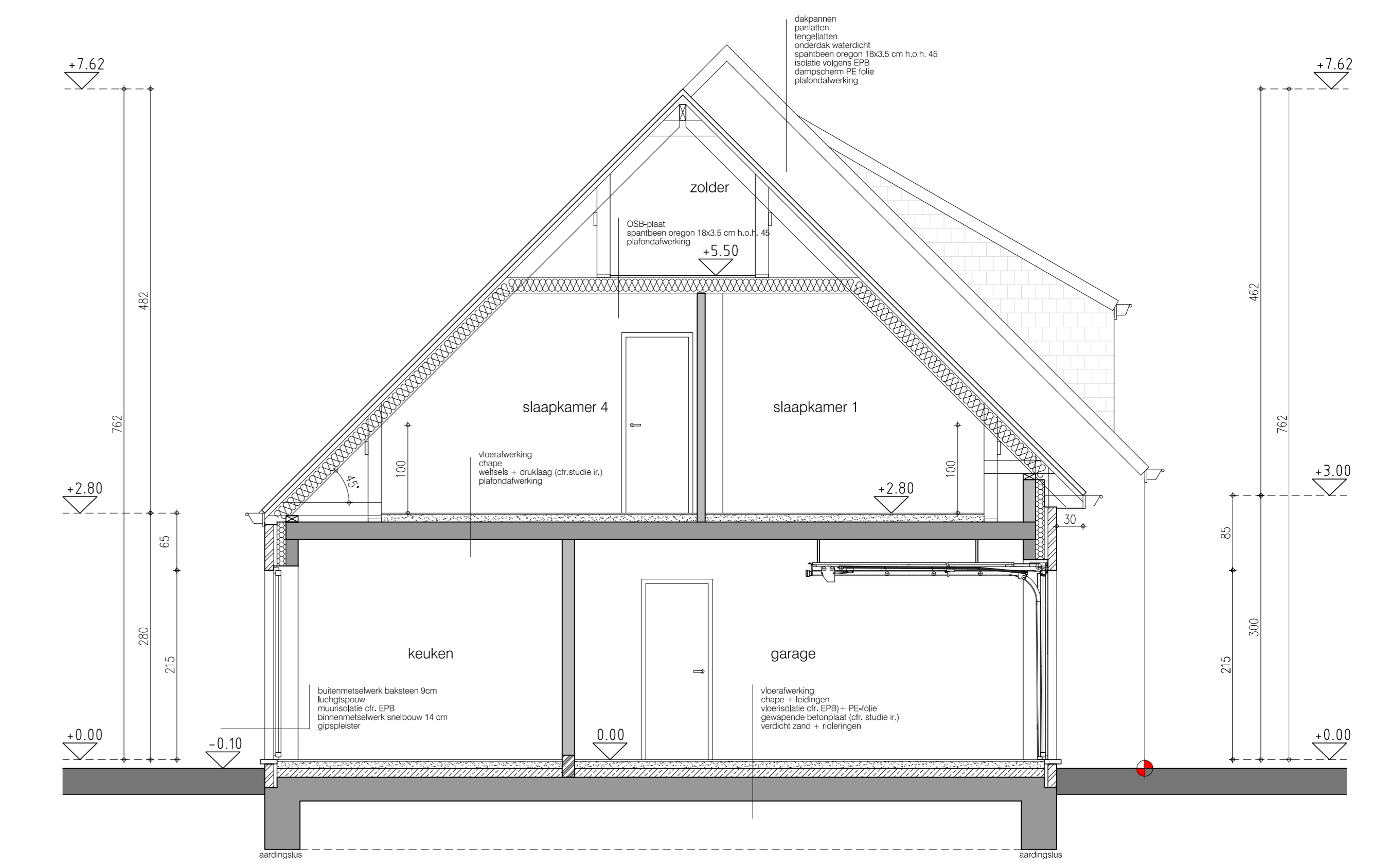
doorsnede 2-2 lot 4
