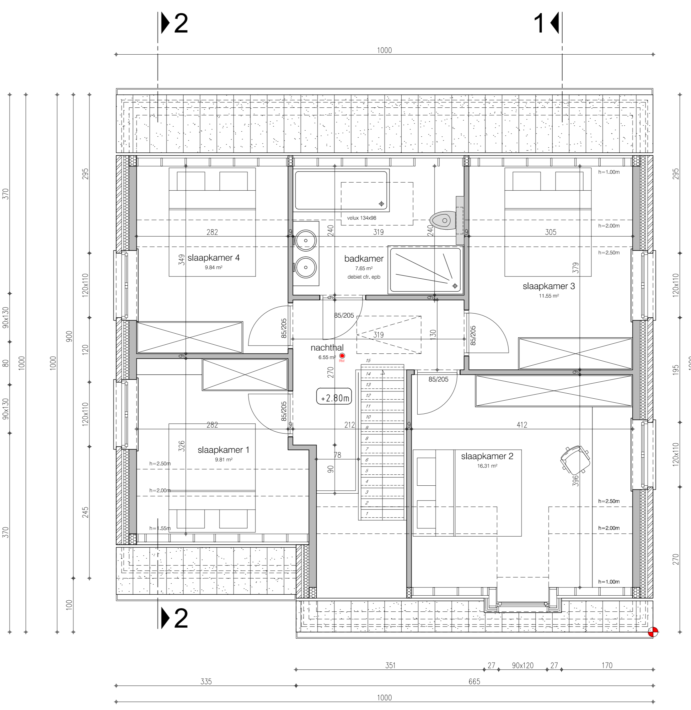
verdiepingsplan lot 4
